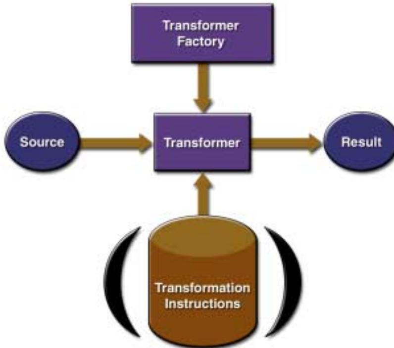
Figure 5–3 XSLT APIs
