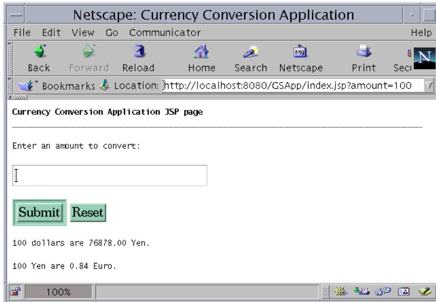
Figure 3–1 ConverterBean Web Client
