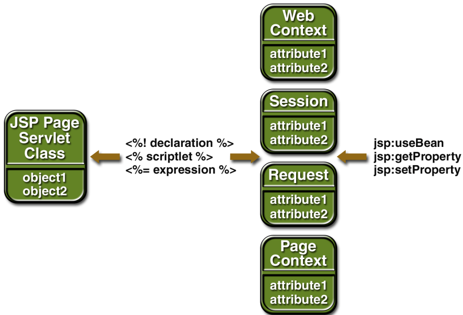
Figure 14-1 Accessing Objects From a JSP Page
