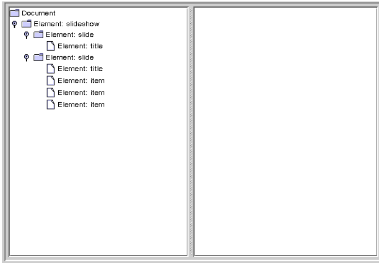
Figure 8 Tree View with a Collapsed Hierarchy
