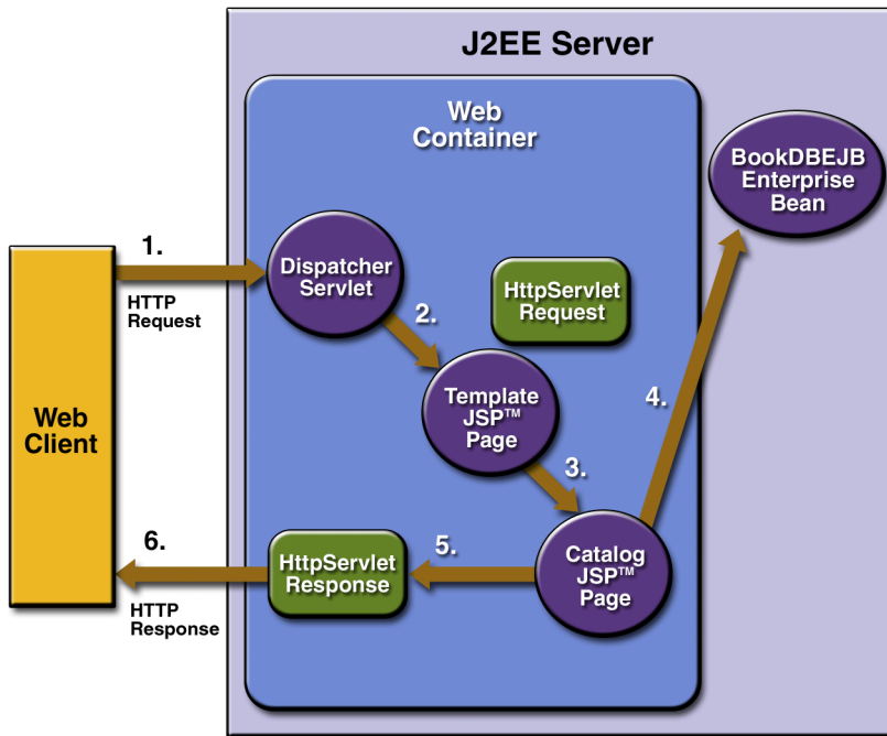
Figure 15–1 Request Flow Through Duke’s Bookstore Components
