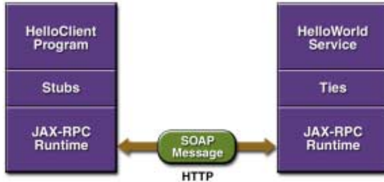
Figure 9–1 The HelloWorld Example at Runtime
