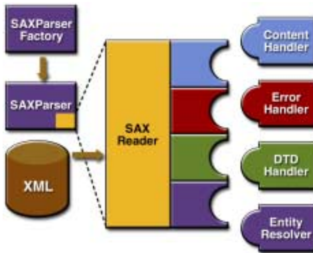
Figure 5-1 SAX APIs
