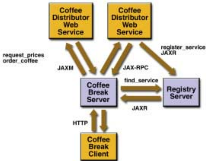
Figure 18–1 Coffee Break Application Flow
