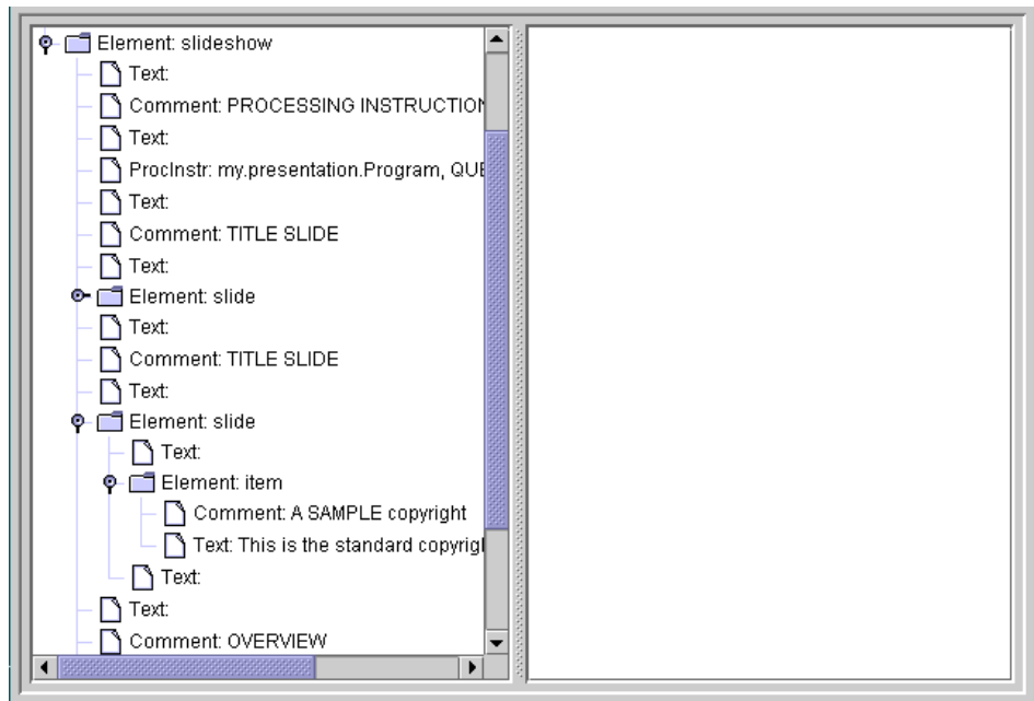
Figure 5 JAXP 1.2 DOM — Item Text Returned from an Entity Reference
