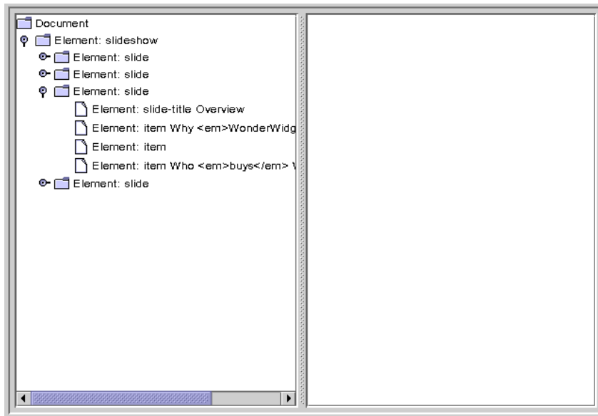
Figure 9 Collapsed Hierarchy Showing Text in Nodes
