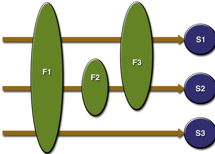
Figure 12–4 Filter to Servlet Mapping
