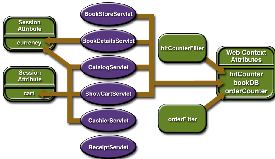
Figure 12–1 Duke’s Bookstore Scoped Attributes
